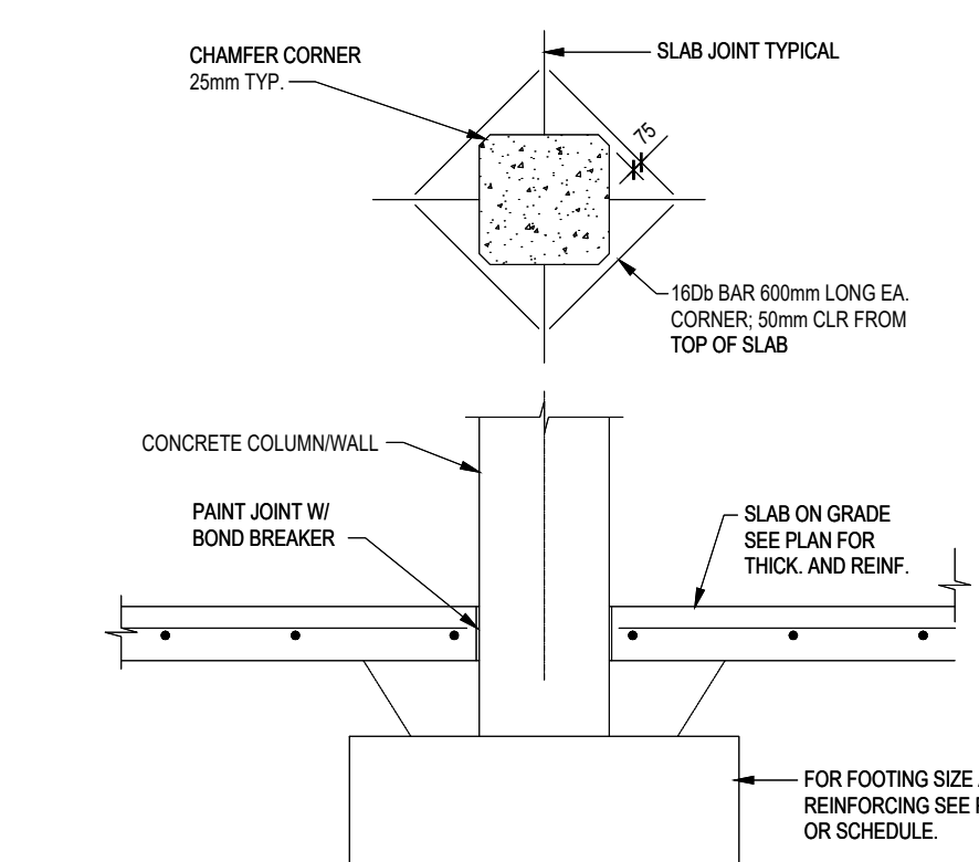
5 SLAB ON GRADE AT COLUMNS
