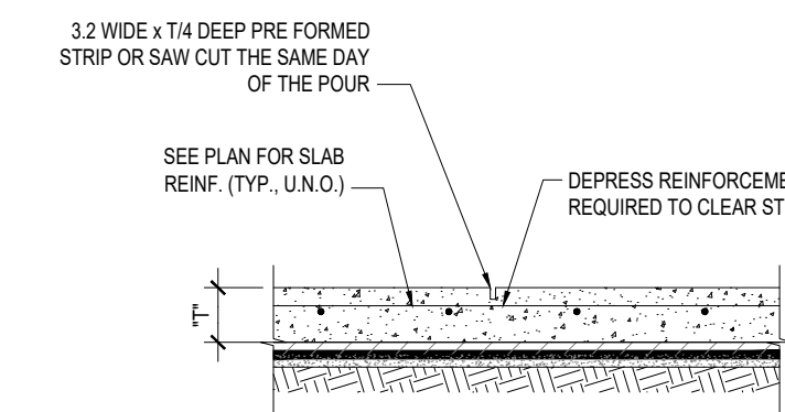
A CONTROL JOINT (WHERE CONTINUOUS POUR IS USED)
