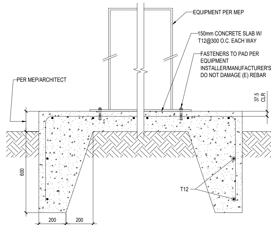
8 EQUIPMENT CONC. PAD ON GRADE
