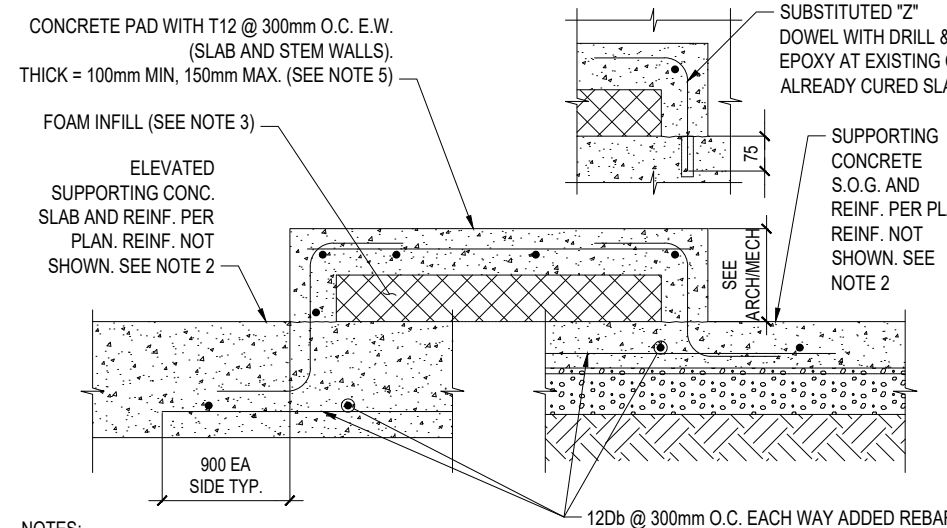
8 EQUIPMENT CONC. PAD ON GRADE
