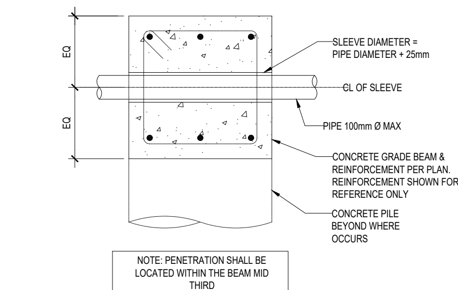
4 TYP. PIPE THROUGH GRADE BEAM
