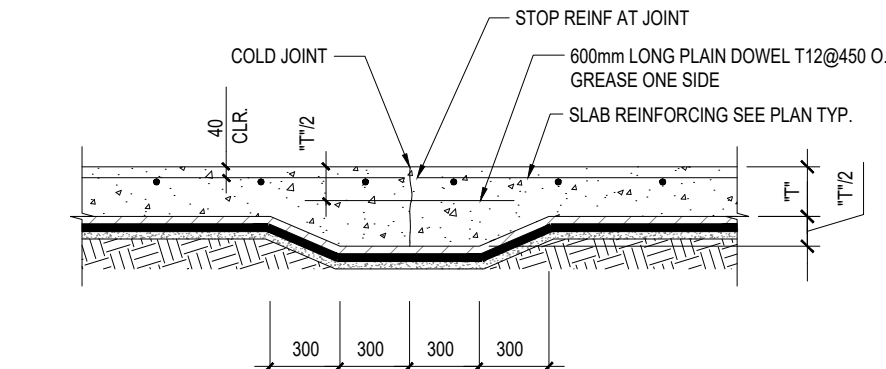
B TYPICAL CONSTRUCTION JOINT
